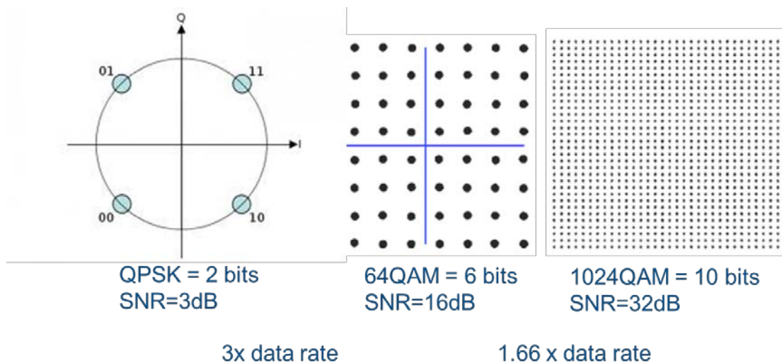
Fig. 2: Modulation vs. Data Rate Improvement
