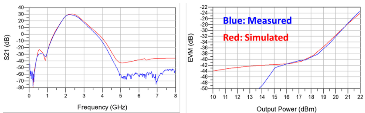
Fig. 9: Small and large-signal performance of the 2G WLAN FEM at 3.3V, 25°C [2]
