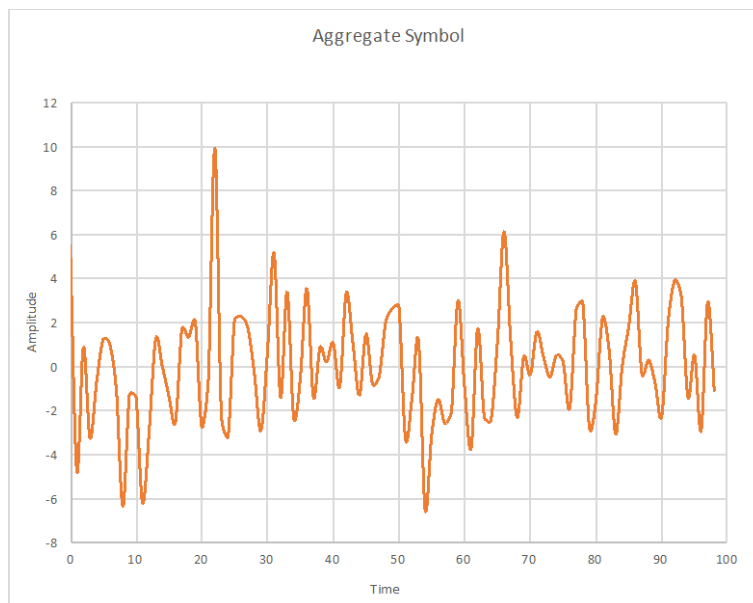
Fig. 4: Combined signal of 48 randomly modulated subcarriers
