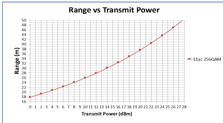
Fig. 1: Range vs. Transmit Power
